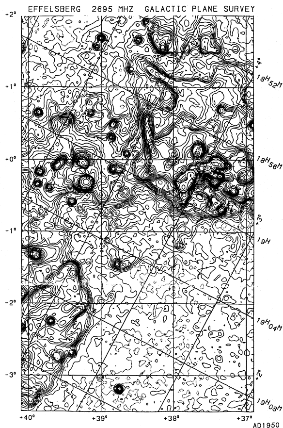
Figure 10: The low-latitude continuum emission at 2.7 GHz for 37^\circ < l < 40^\circ measured with the Effelsberg 100-m telescope (Reich et al. 1990). The image is in Galactic coordinates, and the HPBW \sim 4.3 arcmin.
