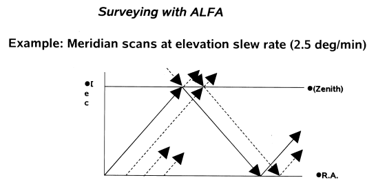
Figure 15: The “zig-zag” scan pattern produced on the sky by NODding the telescope on the prime meridian. Note that the areas of sky north and south of the Arecibo zenith have to be observed at different times as the telescope cannot “scan through the zenith”.
