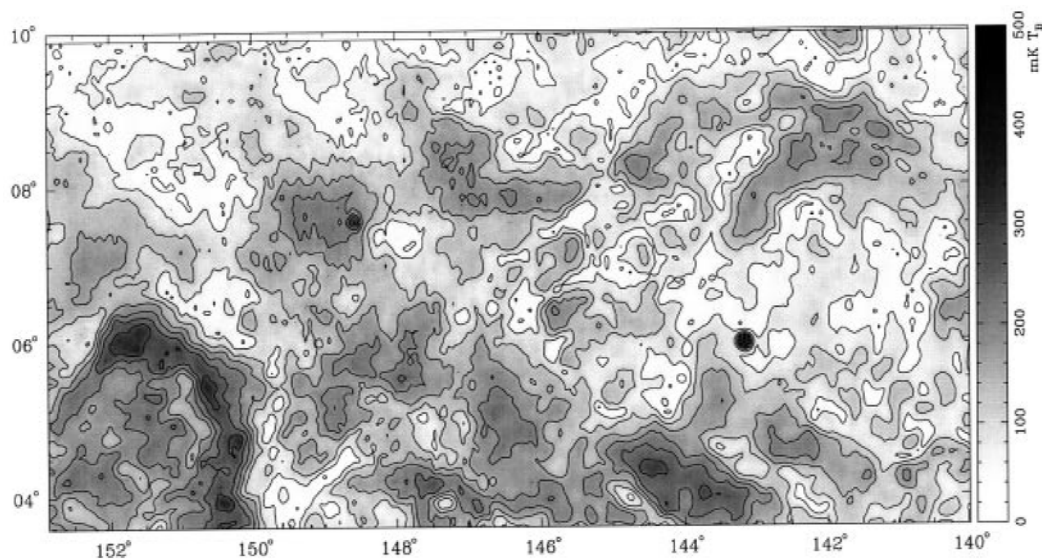
Figure 11: Polarized intensity of the 1.4-GHz emission at l \sim 140^\circ measured with the Effelsberg 100-m telescope (Uyaniker et al. 1999). The image is in Galactic coordinates, and the HPBW \sim 9.4 arcmin.
