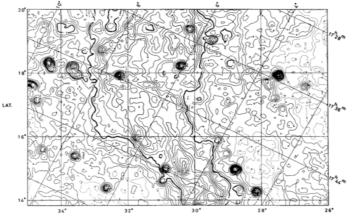
Figure 12: Contour map of the intermediate latitude total-intensity emission from the North Polar Spur at 1.4 GHz made with the Effelsberg telescope (Sofue & Reich 1979). The image is in Galactic coordinates, and the HPBW \sim 10 arcmin.
