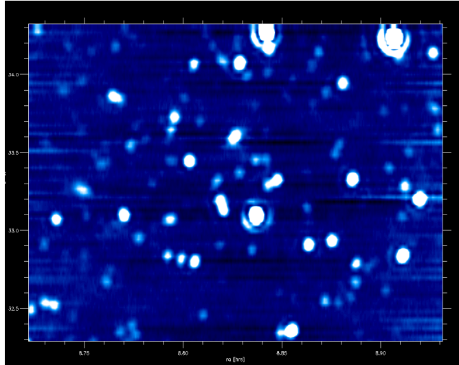
Figure 14: The continuum emission (over a band from 1415–1425 MHz) of a region in the vicinity of the nearby (7.6 Mpc) galaxy NGC 2683. The axes are R.A. (hr), and Dec (deg). Each horizontal strip is normalized to its average flux, leading to the spurious horizontal stripes. The map was obtained in “On-The-Fly” mode with a R.A. drive rate of 6 s per beam, and spaced in Dec each 1.65 arcmin. The map covers 2^\circ \times 1.5^\circ .
